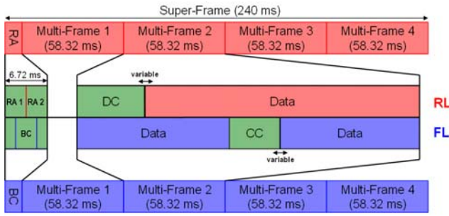
Figure 1: L-DACS1 framing structure.
